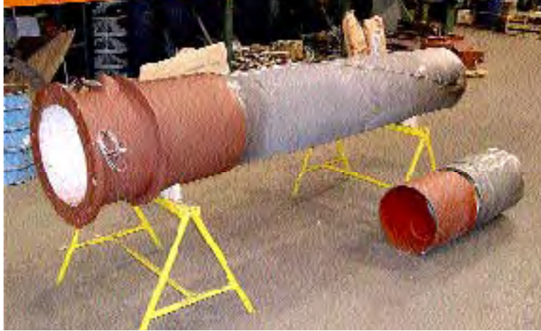
CERAMIC LINED COAL NOZZLE
